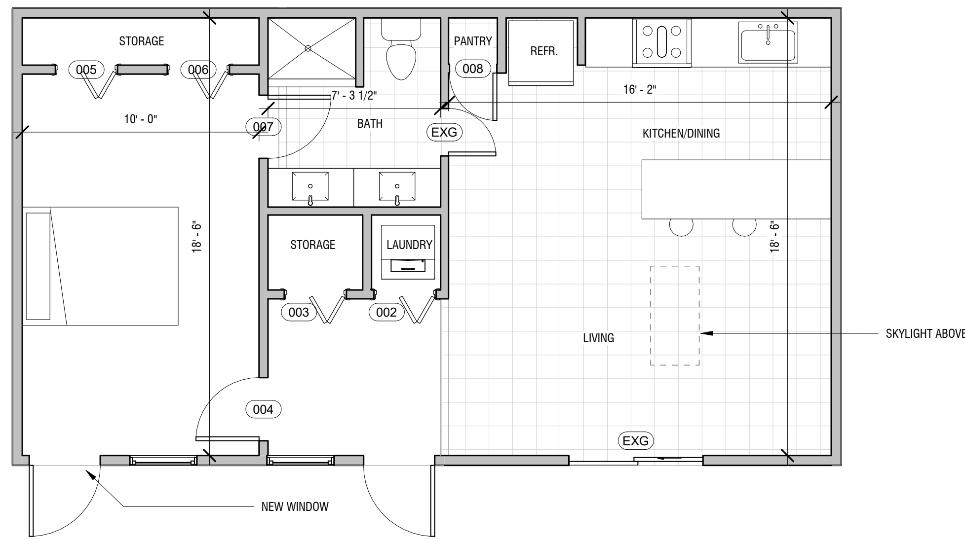
3 BACK APARTMENT 1/4" = 1'-0"
