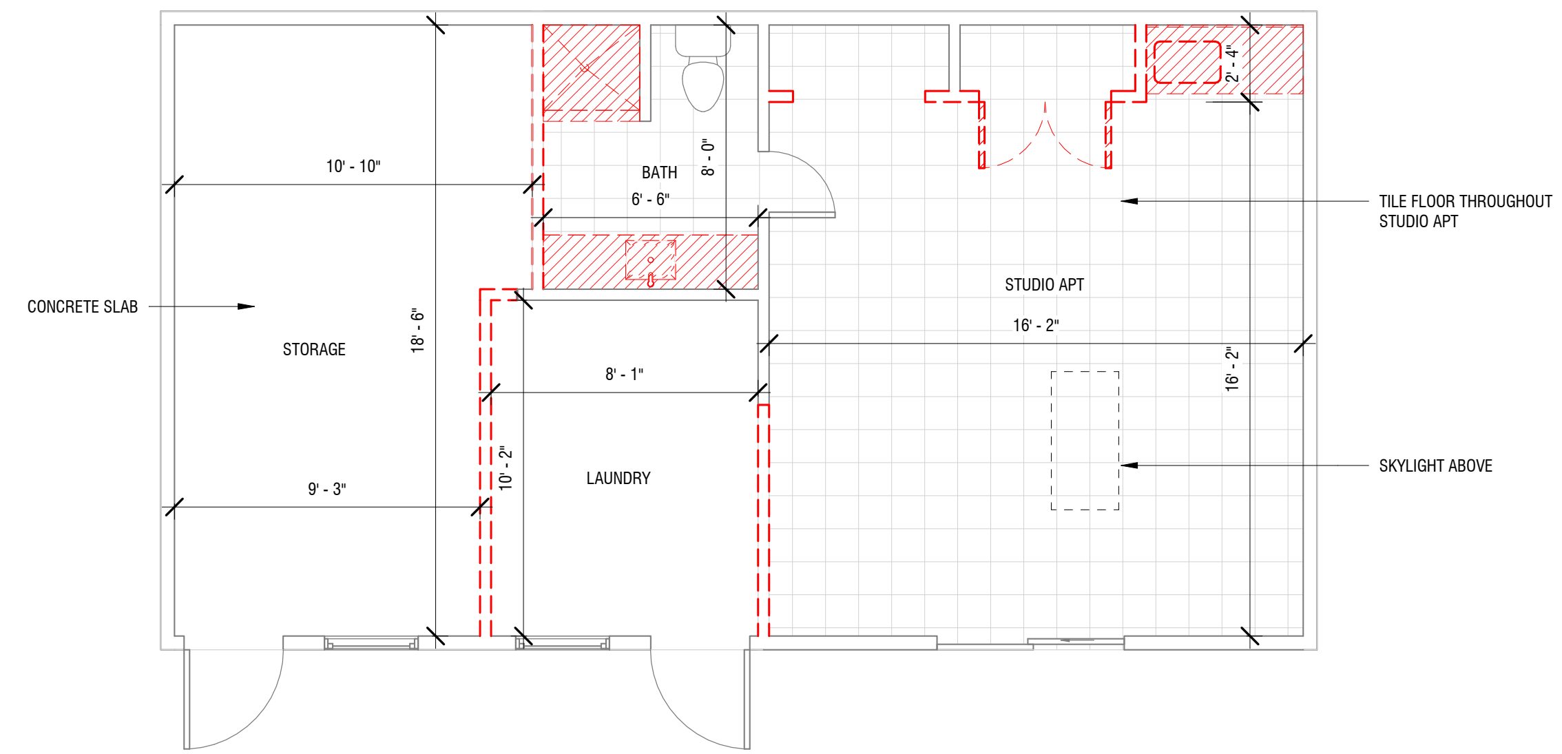
1 BACK APARTMENT DEMO PLAN 1/4" = 1'-0"
